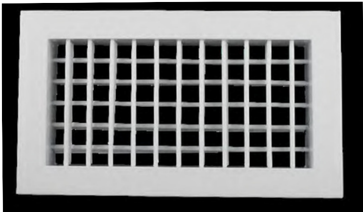
D D G-A1 material: aluminum standard color: white Ral9016/9010 blades are adjustable customized size upon request
