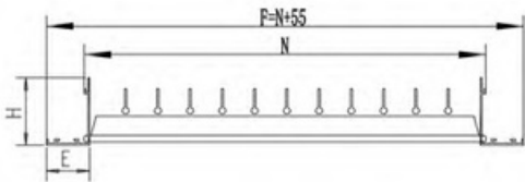
D D G-A1 material: aluminum standard color: white Ral9016/9010 blades are adjustable customized size upon request
