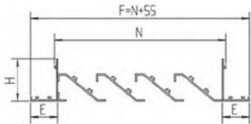
FL-A material:aluminum white Ral9016 / 9010; any size is available
