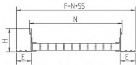
EG-F material: aluminum standard color: white Ral9016 / 9010 12.7x12.7mm core, 90 degree core customized size upon request
